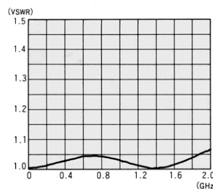
Fig. 1 VSWR for BCP-C3B
